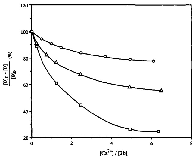
Figure 6. Decrease of the CD intensity of monosaccharide-2b complexes: D-glucose (O), D-talose (Δ), D-allose (□). [2b] = 1.63 × 10 -3 M. pH = 11.6 with 0.2% choline hydroxide as the base in 9:1 CH 3 OH:H 2 O at 25 °C. [θ] 0 and [θ] are the CD intensity in the absence or in the presence of calcium perchlorate.
