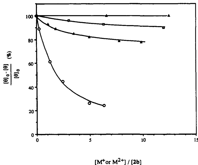
Figure 5. Decrease of the CD intensity of D-allose-2b complex in the presence of metal perchlorate: Ca 2+ (O), K + (Δ), Mg 2+ (□), [Li + , Na + , Rb + , Cs + ] (▲). [2b] = 1.63 × 10 -3 M. pH = 11.6 with 0.2% choline hydroxide as the base in 9:1 CH 3 OH:H 2 O at 25 °C. [θ] 0 and [θ] are the CD intensity in the absence or in the presence of metal salt.
