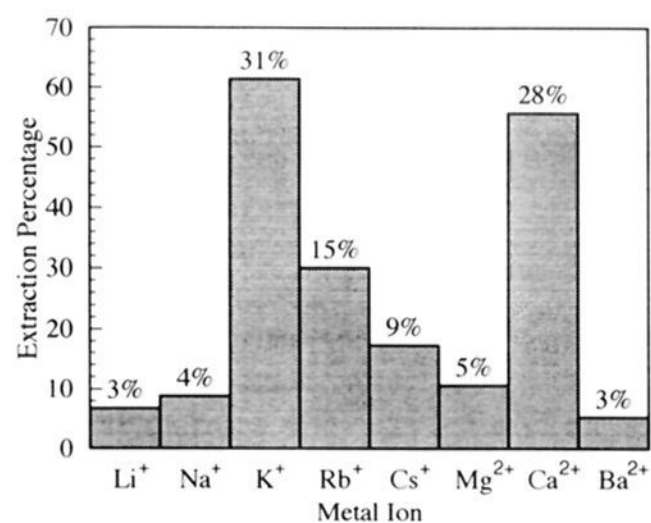
Figure 3. Percentage extraction of metal picrates into \text{CH}_2\text{Cl}_2 at 25 °C by compound 4a .
