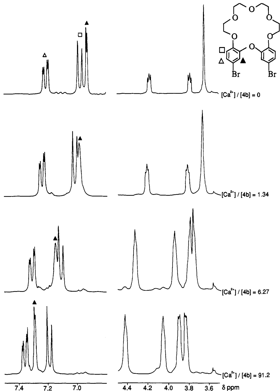
Figure 4. Titration of the ^1\text{H} NMR (300 MHz) spectra of 4b ( 1.45 \times 10^{-2} M) with \text{Ca}(\text{ClO}_4)_2 \cdot 4\text{H}_2\text{O} in 2:1 \text{CD}_3\text{OD}:\text{CDCl}_3 at 25^\circ\text{C} .
